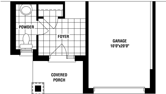
PART. GROUND FLOOR PLAN ELEV. 'C'
