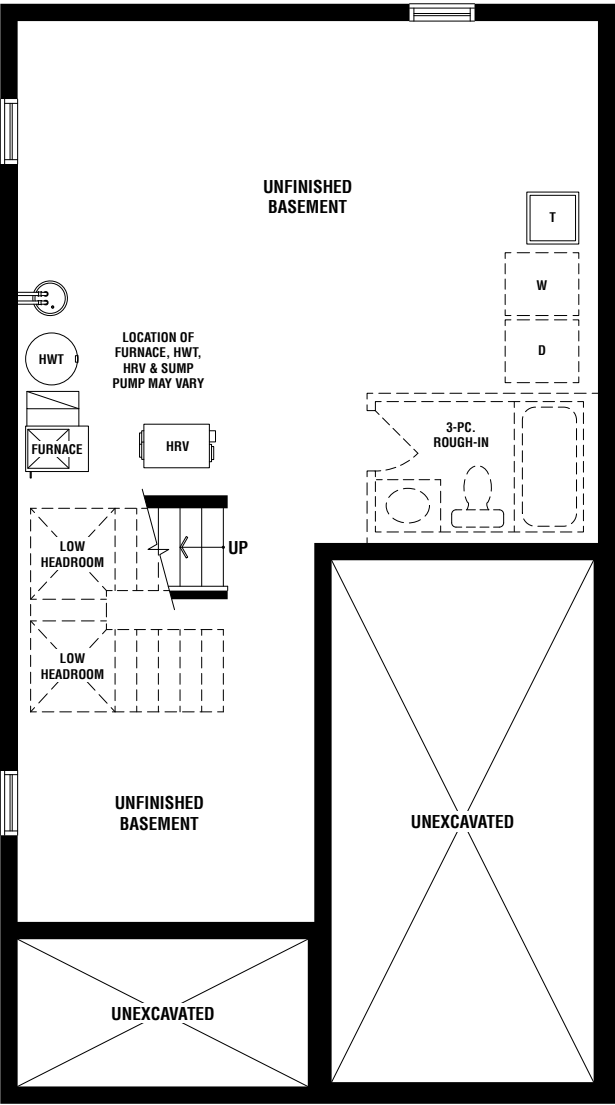
BASEMENT PLAN ELEV. 'A'
