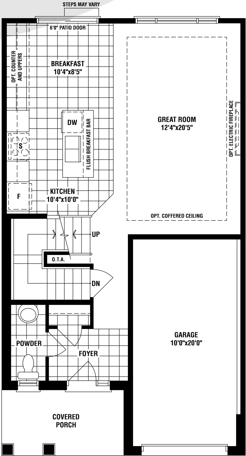
GROUND FLOOR PLAN ELEV. 'A'
