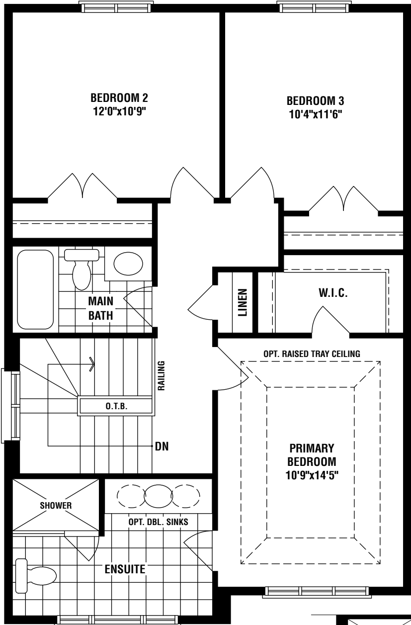
SECOND FLOOR PLAN ELEV. 'A'
